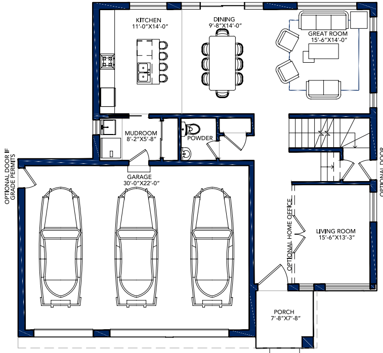
FIRST FLOOR AREA = 1073 SQ. FT
