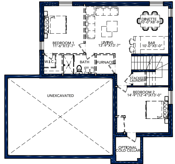
OPTIONAL FINISHED BASEMENT FLOOR AREA = 1088 SQ. FT
