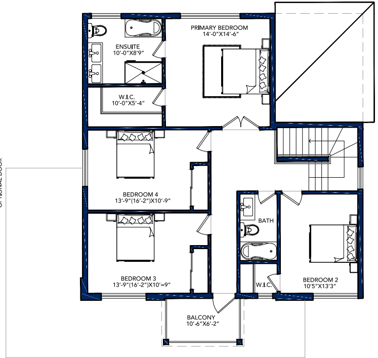
SECOND FLOOR AREA = 1260 SQ. FT
