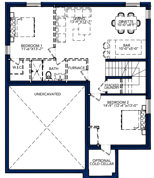
OPTIONAL FINISHED BASEMENT BASEMENT FLOOR AREA = 1088 SQ FT
