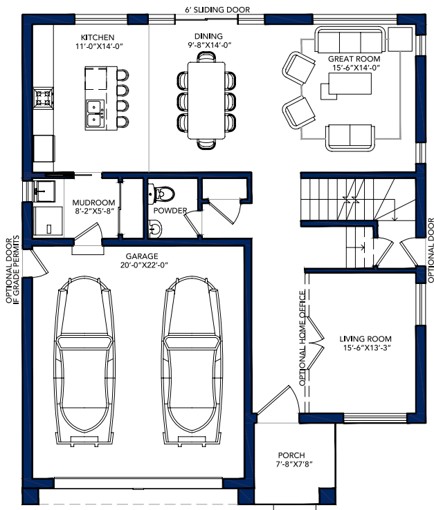
FIRST FLOOR AREA = 1073 SQ FT
