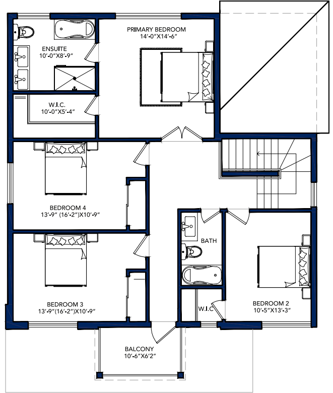
SECOND FLOOR AREA = 1260 SQ FT
