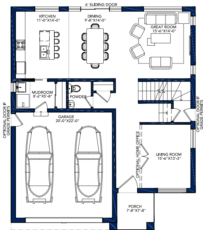
FIRST FLOOR AREA = 1073 SQ FT
